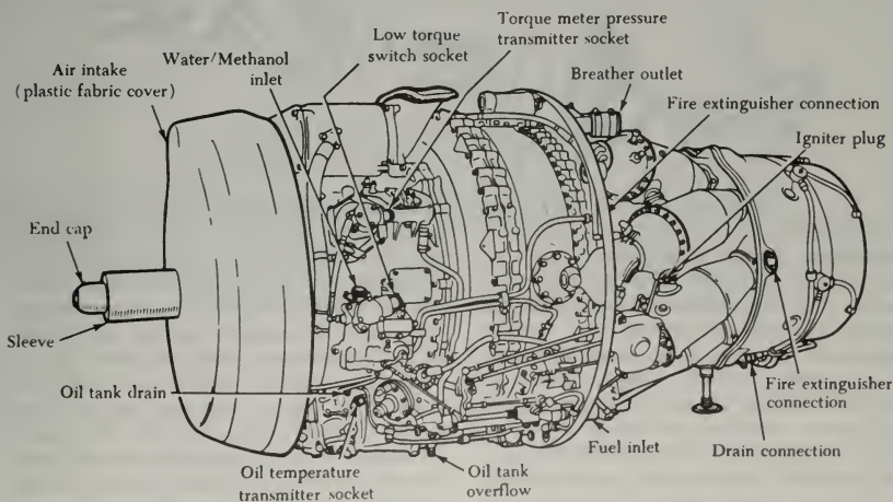
FIGURE 1-43. Can-type combustion chamber arrangement.
